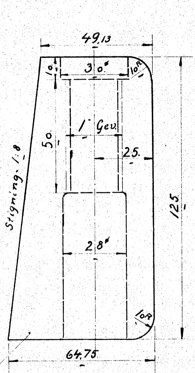
1. Kile for Drivstang
